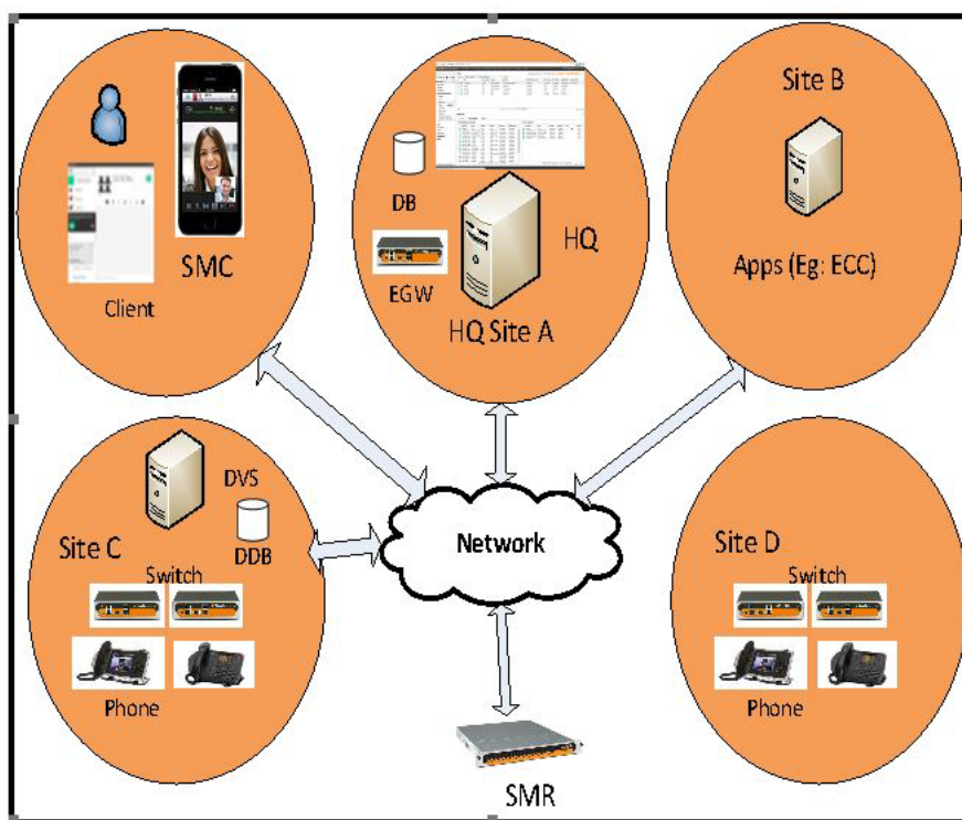
Figure 4: A typical Mitel Connect ONSITE Deployment
