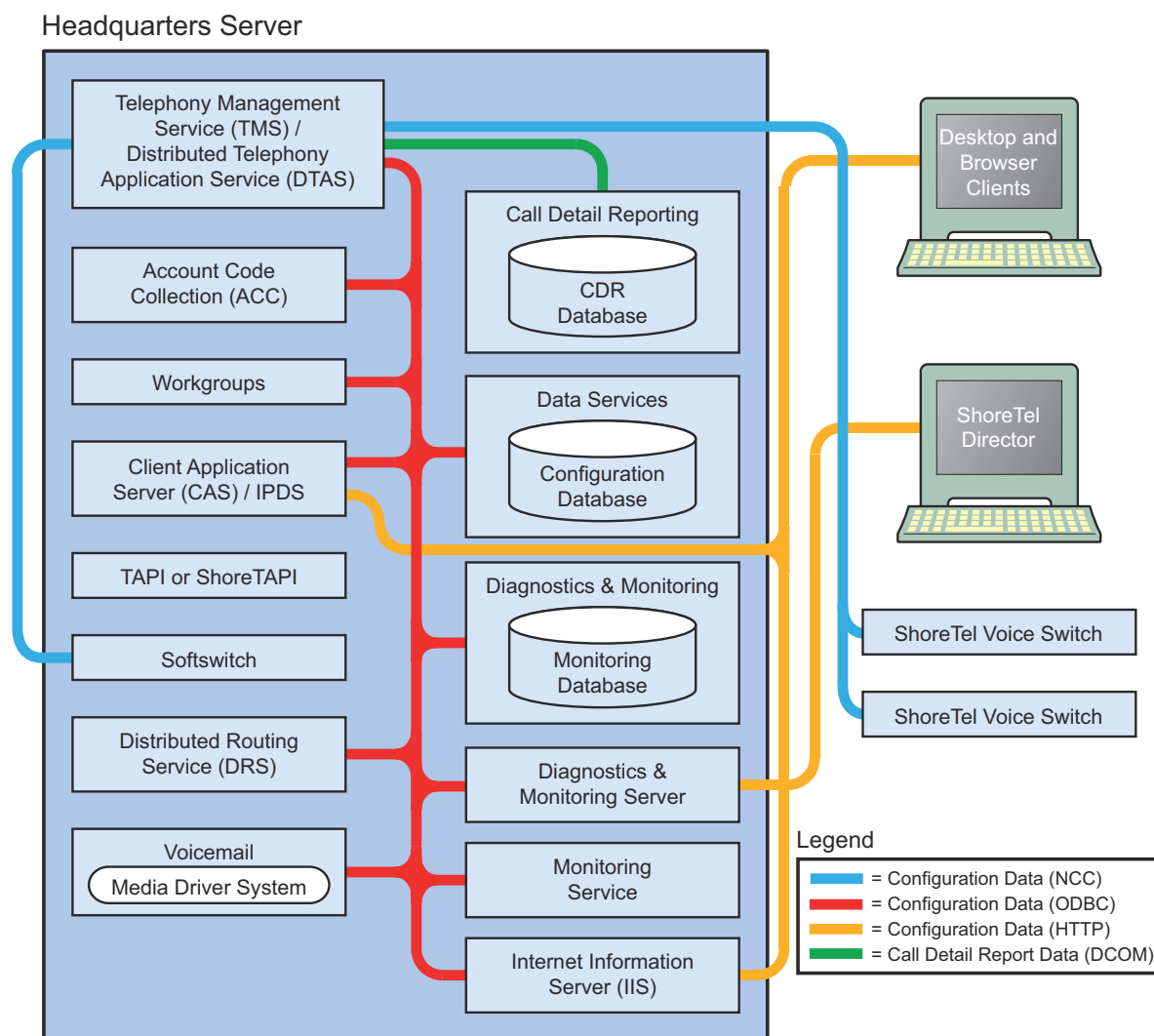
Figure 5: Server Database Communications
