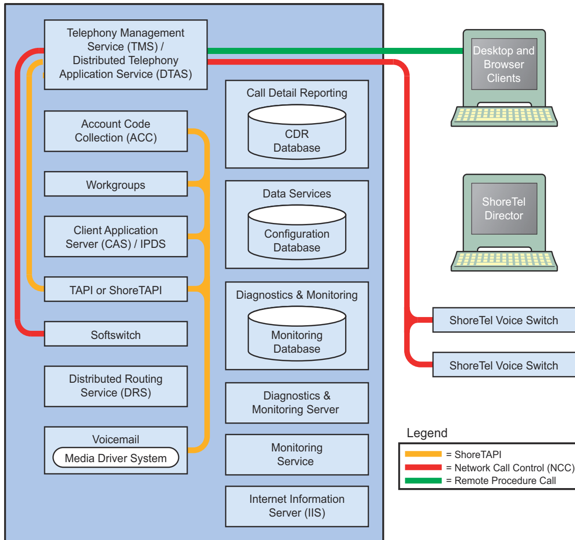
Figure 6: Server TAPI Communications
