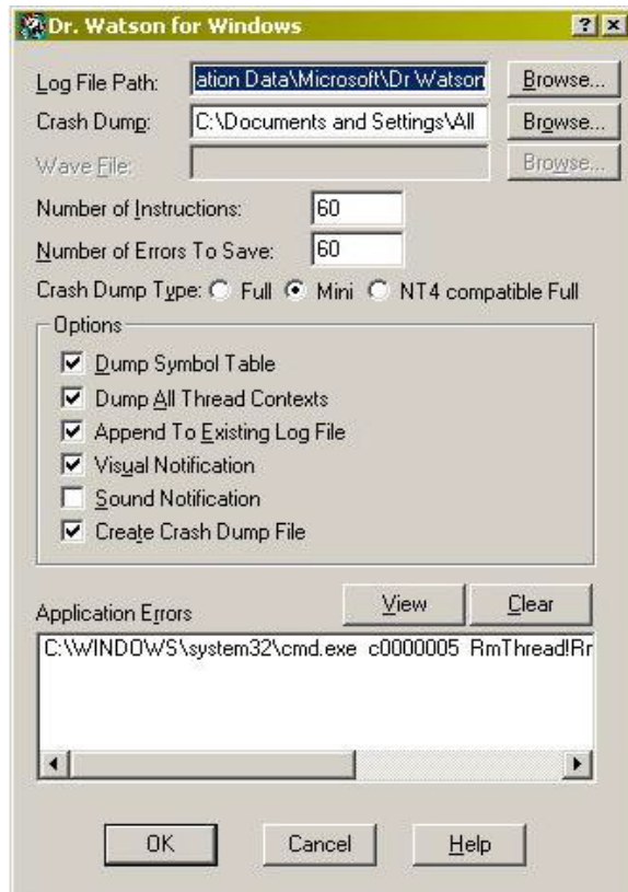
Figure 9: Configuring Dr. Watson
