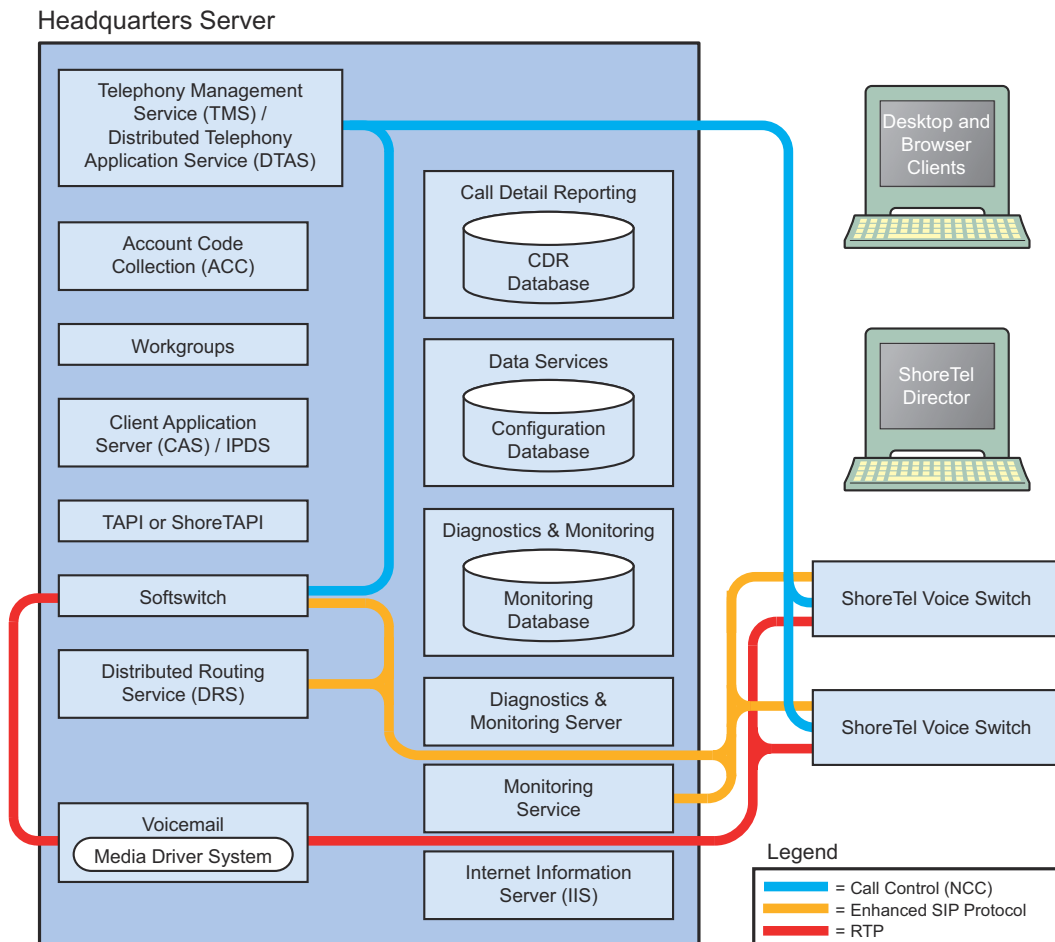
Figure 7: Server Call Control and Media Communications
